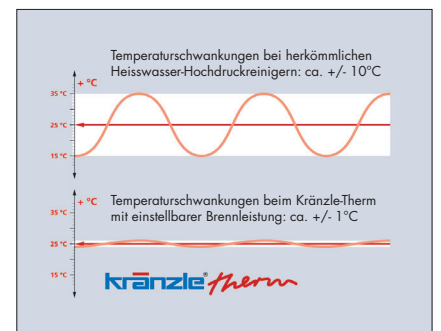
Thermostat-Regelung
